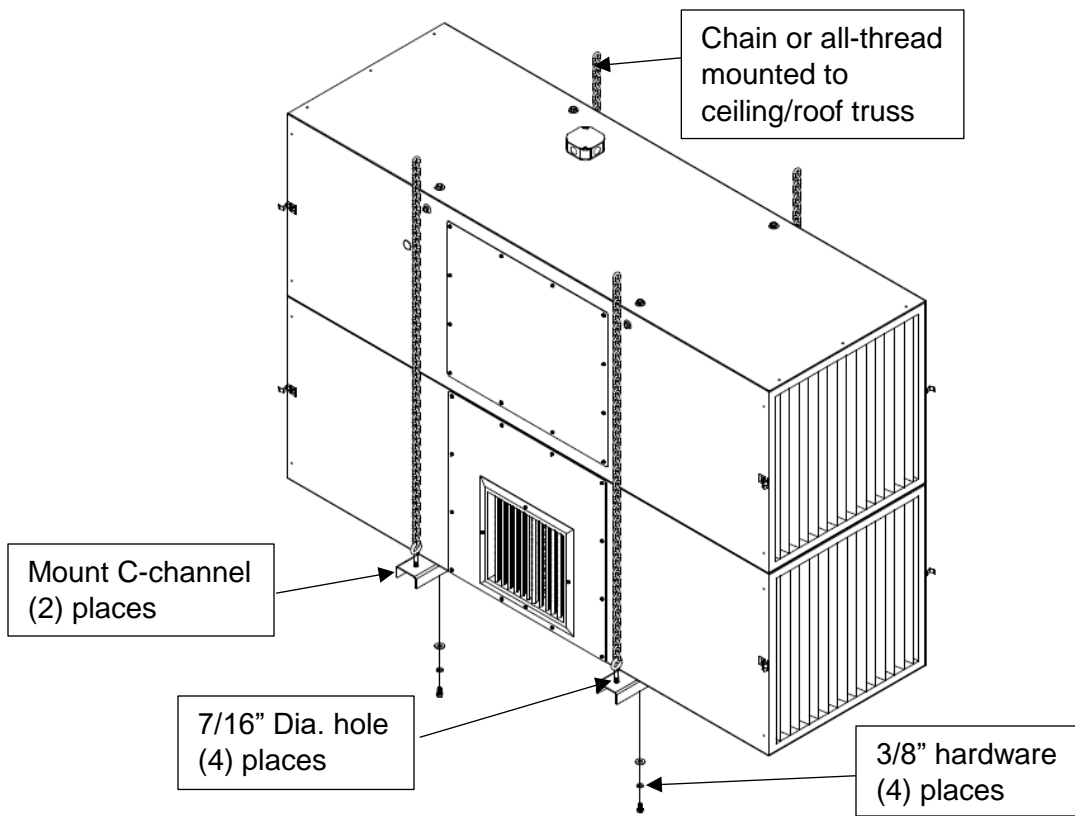
FIG. 4 – Vertical configuration.
